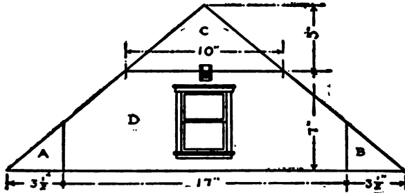
FIG. 240. — Front Gable-End.
